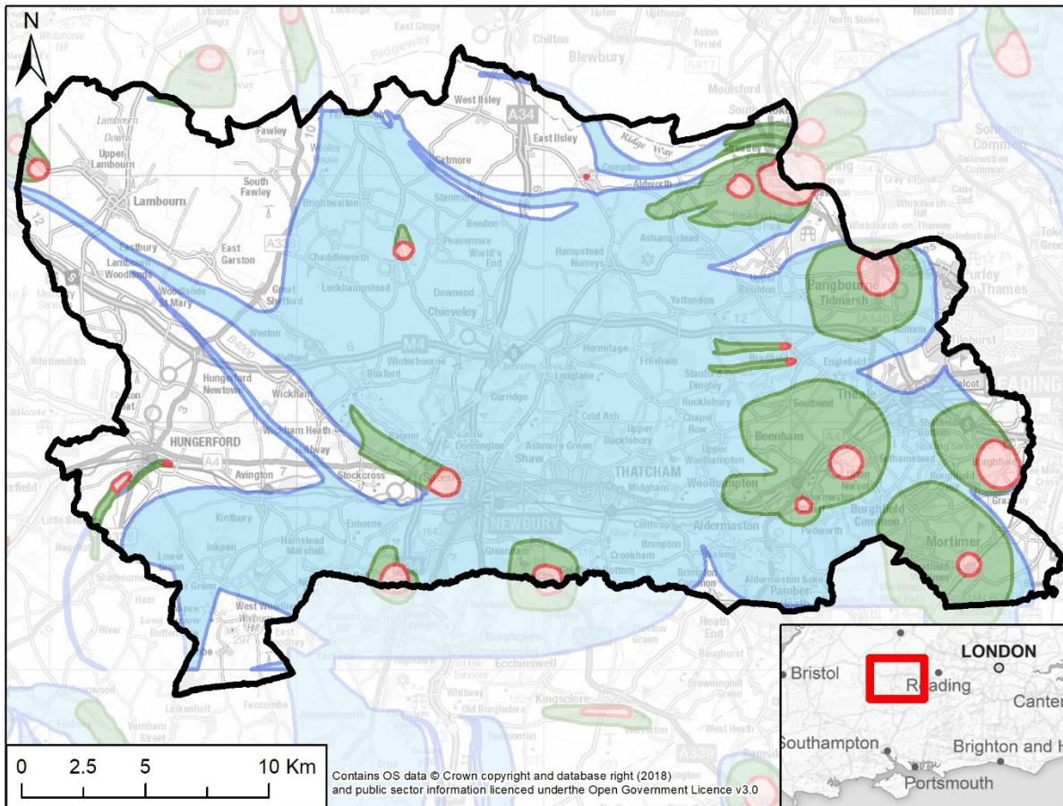
Figure 4-3: Groundwater Source Protection Zones in West Berkshire
